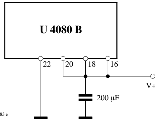
Figure 14. Regulated power supply
